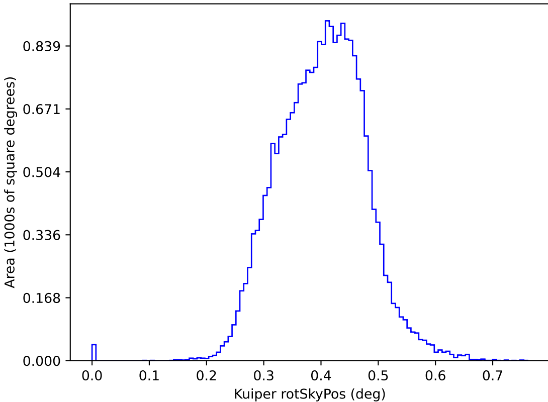
roll_pause_mjdp120_v3.4_10yrs y: Kuiper rotSkyPos
