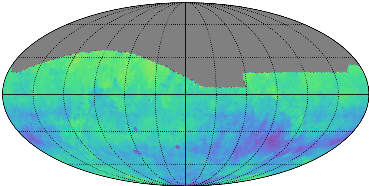
roll_pause_mjdp120_v3.4_10yrs i: Kuiper rotSkyPos
