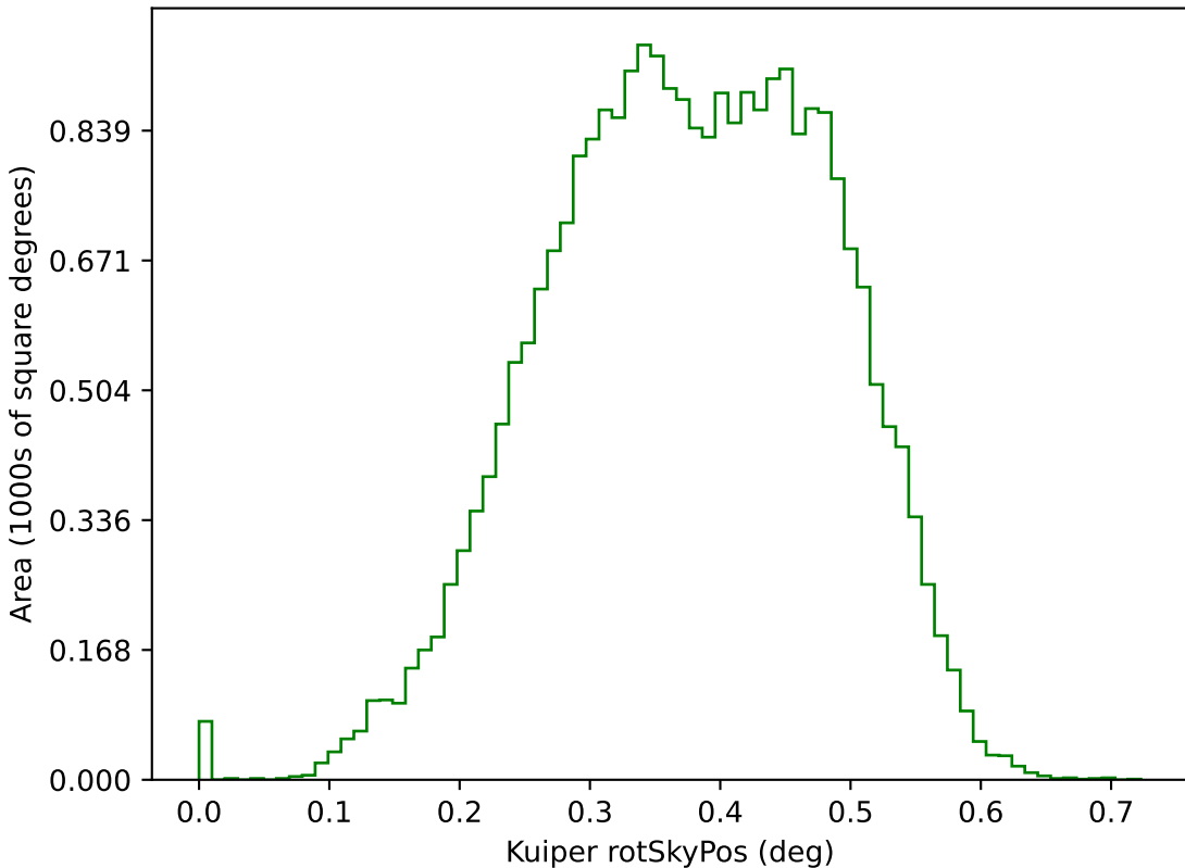
roll_pause_mjdp120_v3.4_10yrs g: Kuiper rotSkyPos
