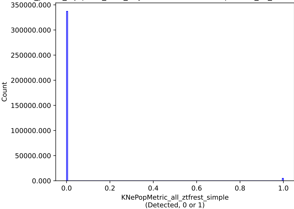
roll_pause_mjdp120_v3.4_10yrs all models: KNePopMetric_all_ztfrest_simple
