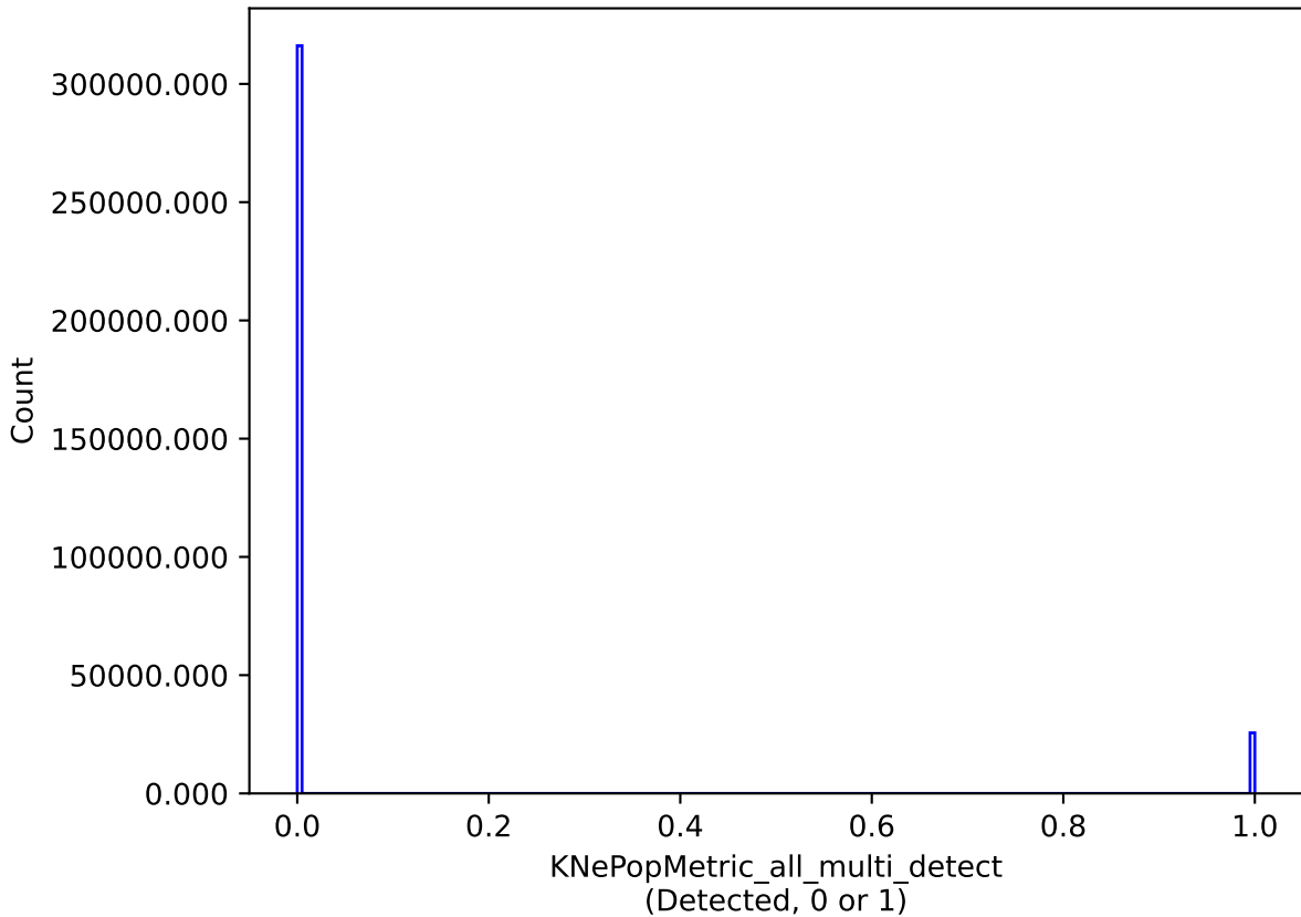
roll_pause_mjdp120_v3.4_10yrs all models: KNePopMetric_all_multi_detect
