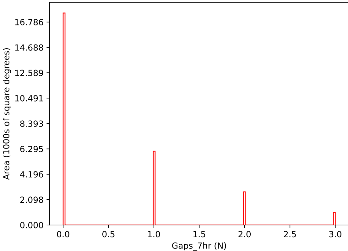
roll_pause_mjdp120_v3.4_10yrs i band: Gaps_7hr
