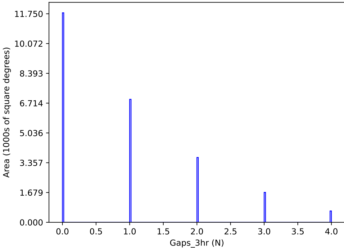
roll_pause_mjdp120_v3.4_10yrs y band: Gaps_3hr
