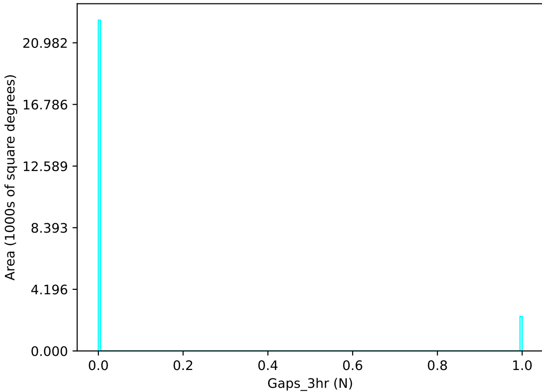
roll_pause_mjdp120_v3.4_10yrs u band: Gaps_3hr
