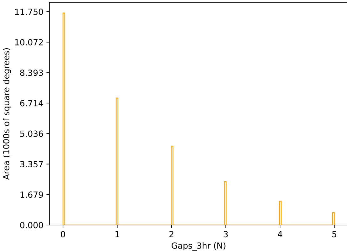
roll_pause_mjdp120_v3.4_10yrs r band: Gaps_3hr
