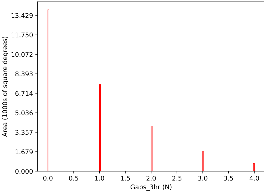
roll_pause_mjdp120_v3.4_10yrs i band: Gaps_3hr
