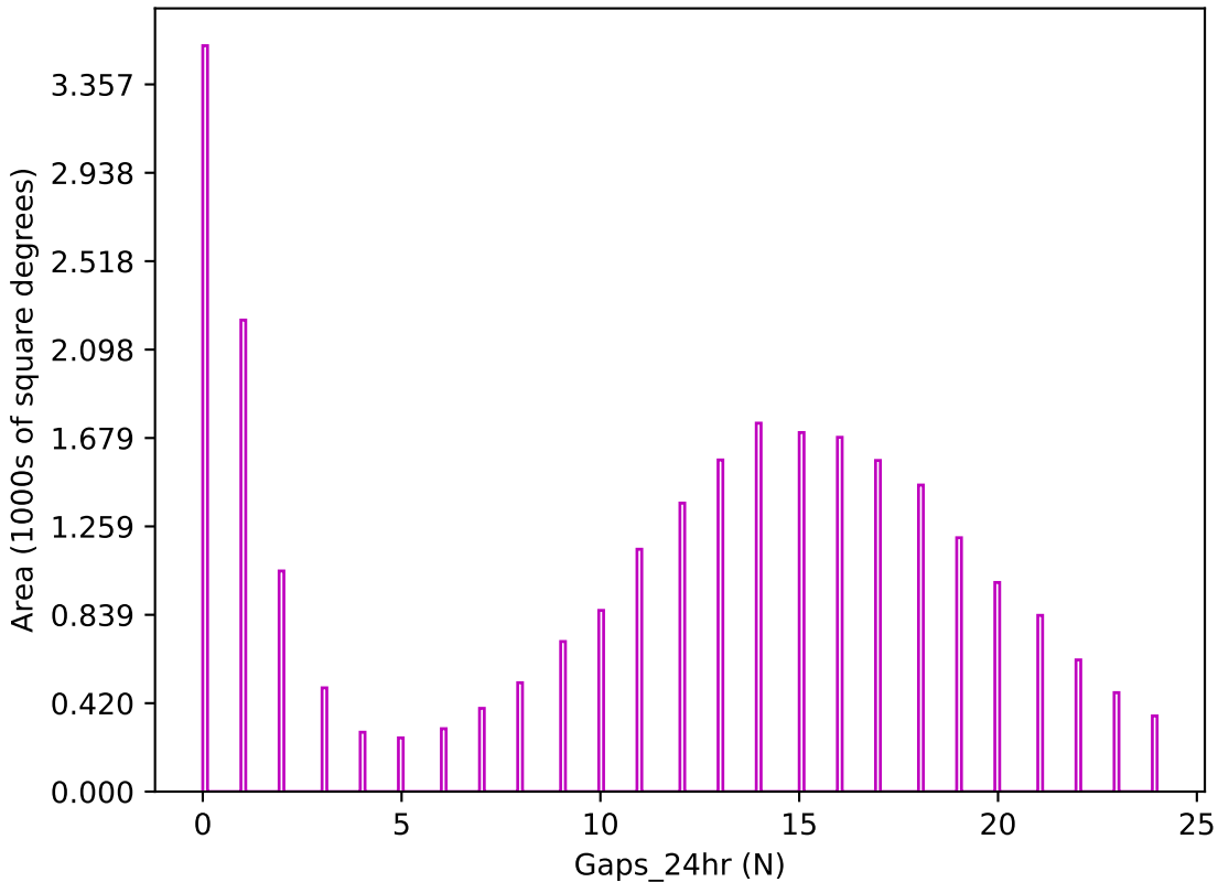
roll_pause_mjdp120_v3.4_10yrs z band: Gaps_24hr
