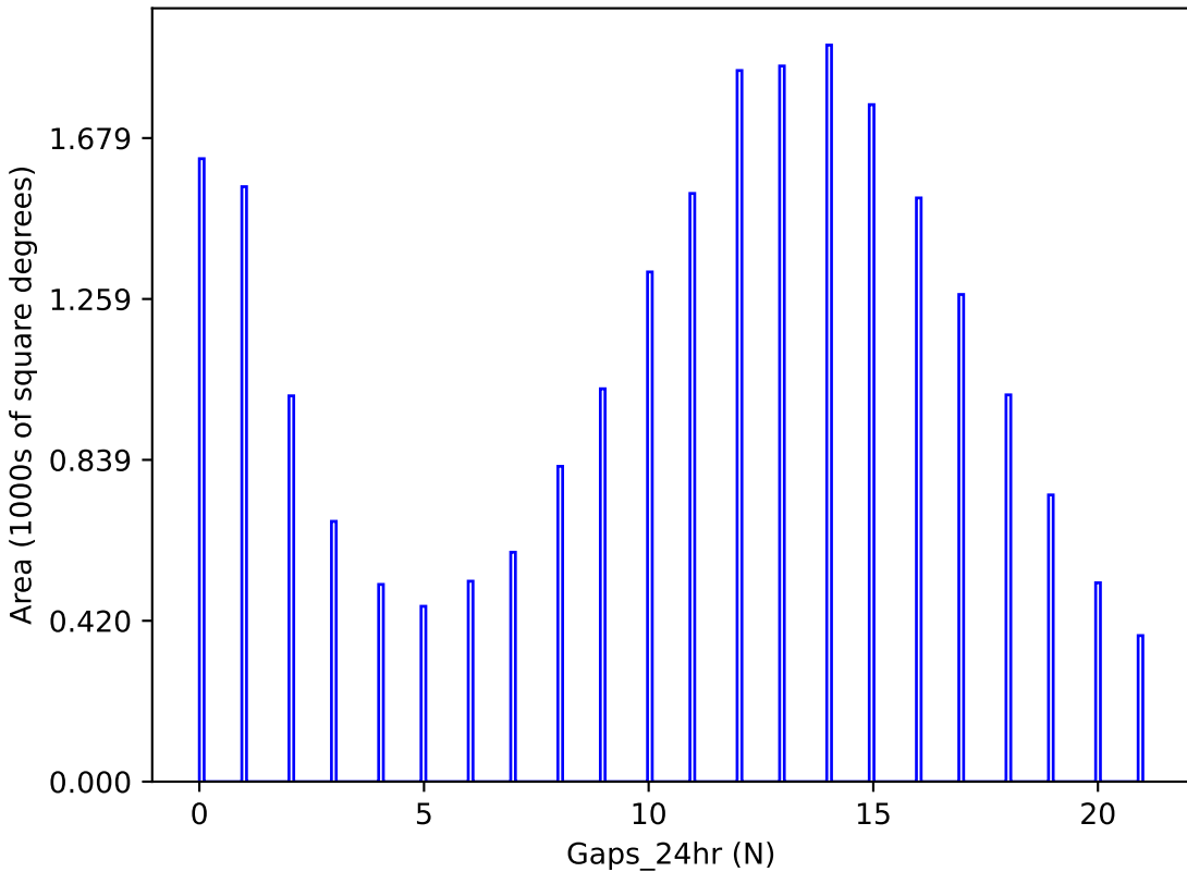
roll_pause_mjdp120_v3.4_10yrs y band: Gaps_24hr
