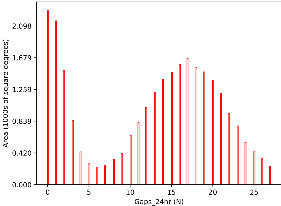
roll_pause_mjdp120_v3.4_10yrs i band: Gaps_24hr
