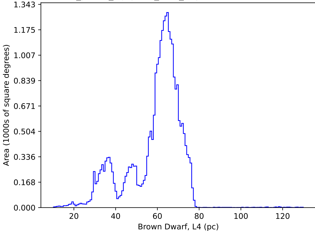
roll_pause_mjdp120_v3.4_10yrs : Brown Dwarf, L4
