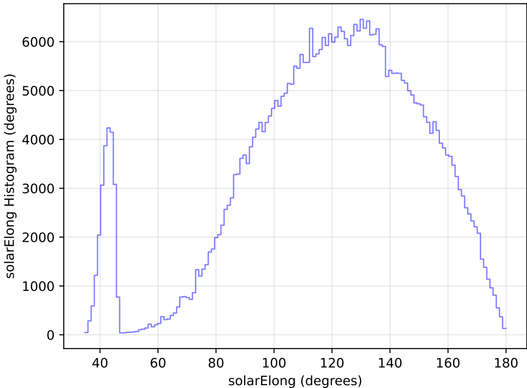
roll_pause_mjdp120_v3.4_10yrs WFD z band: solarElong Histogram
