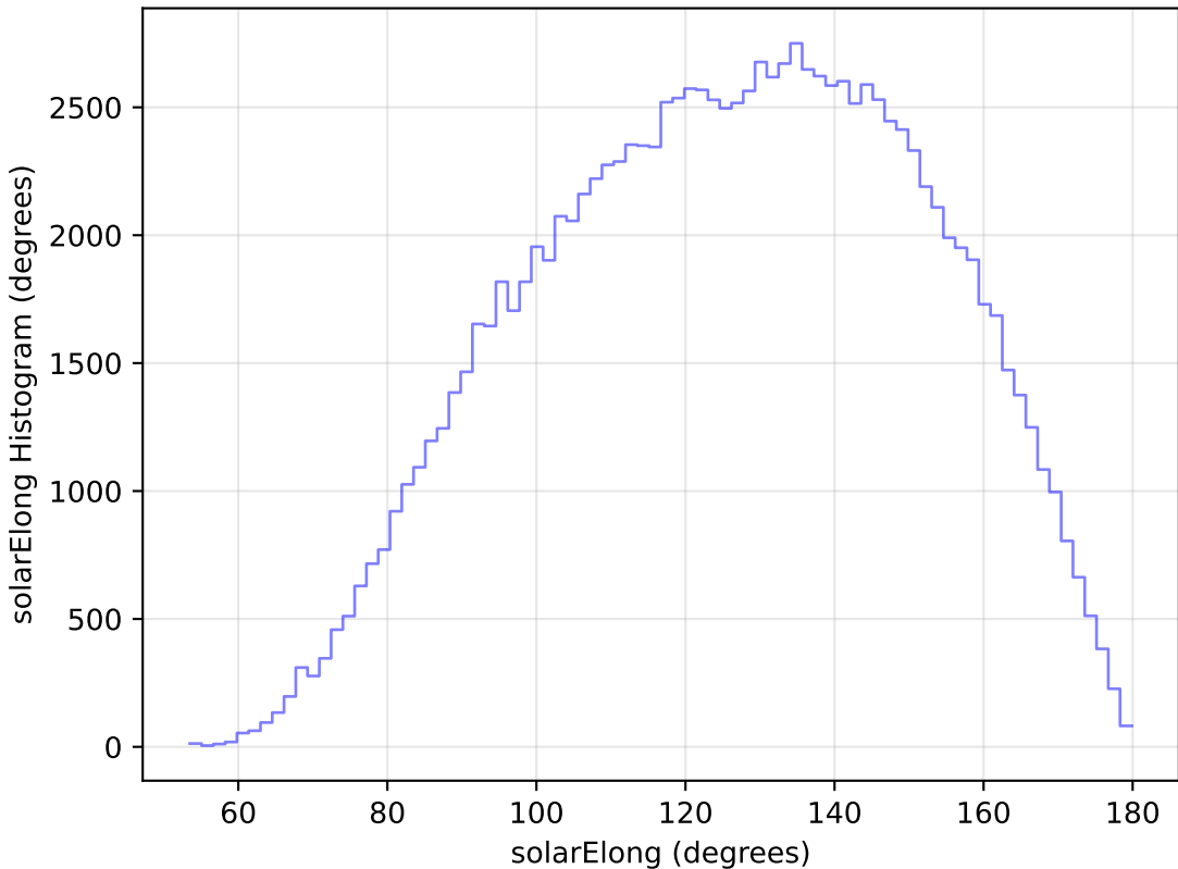
roll_pause_mjdp120_v3.4_10yrs WFD u band: solarElong Histogram
