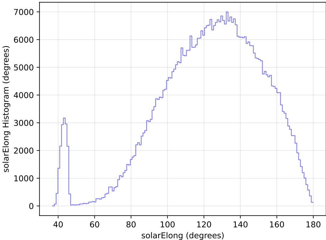
roll_pause_mjdp120_v3.4_10yrs WFD r band: solarElong Histogram
