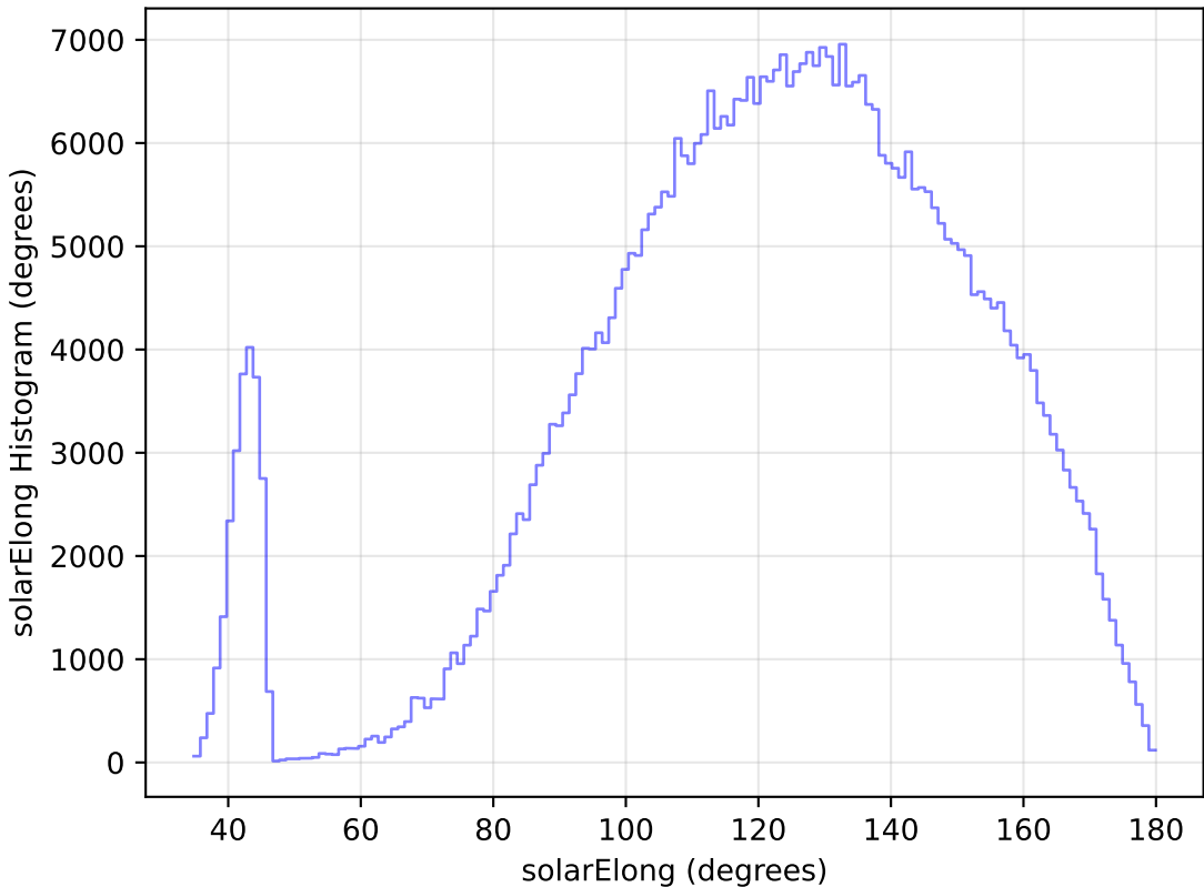
roll_pause_mjdp120_v3.4_10yrs WFD i band: solarElong Histogram
