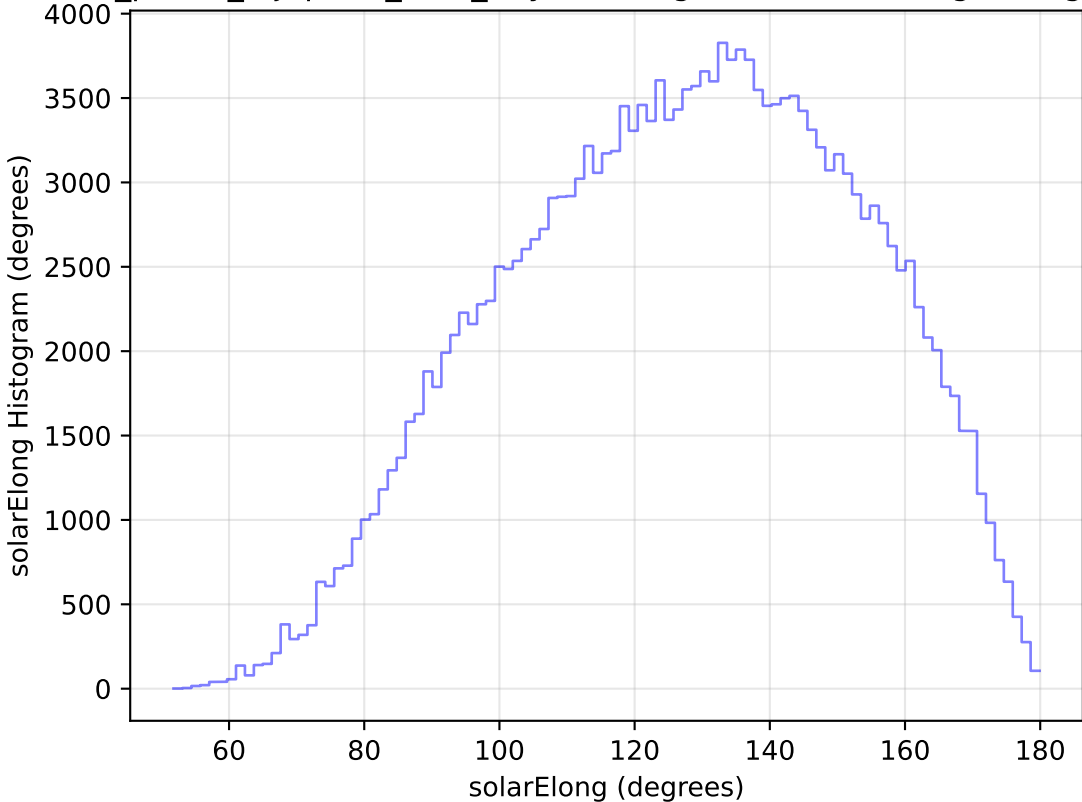
roll_pause_mjdp120_v3.4_10yrs WFD g band: solarElong Histogram
