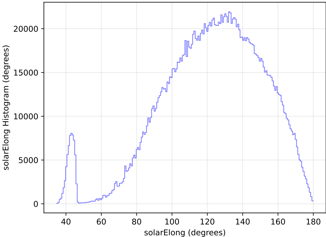
roll_pause_mjdp120_v3.4_10yrs WFD all bands: solarElong Histogram
