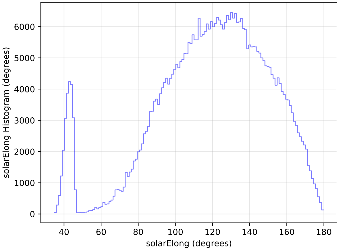
roll_pause_mjdp120_v3.4_10yrs All sky z band: solarElong Histogram
