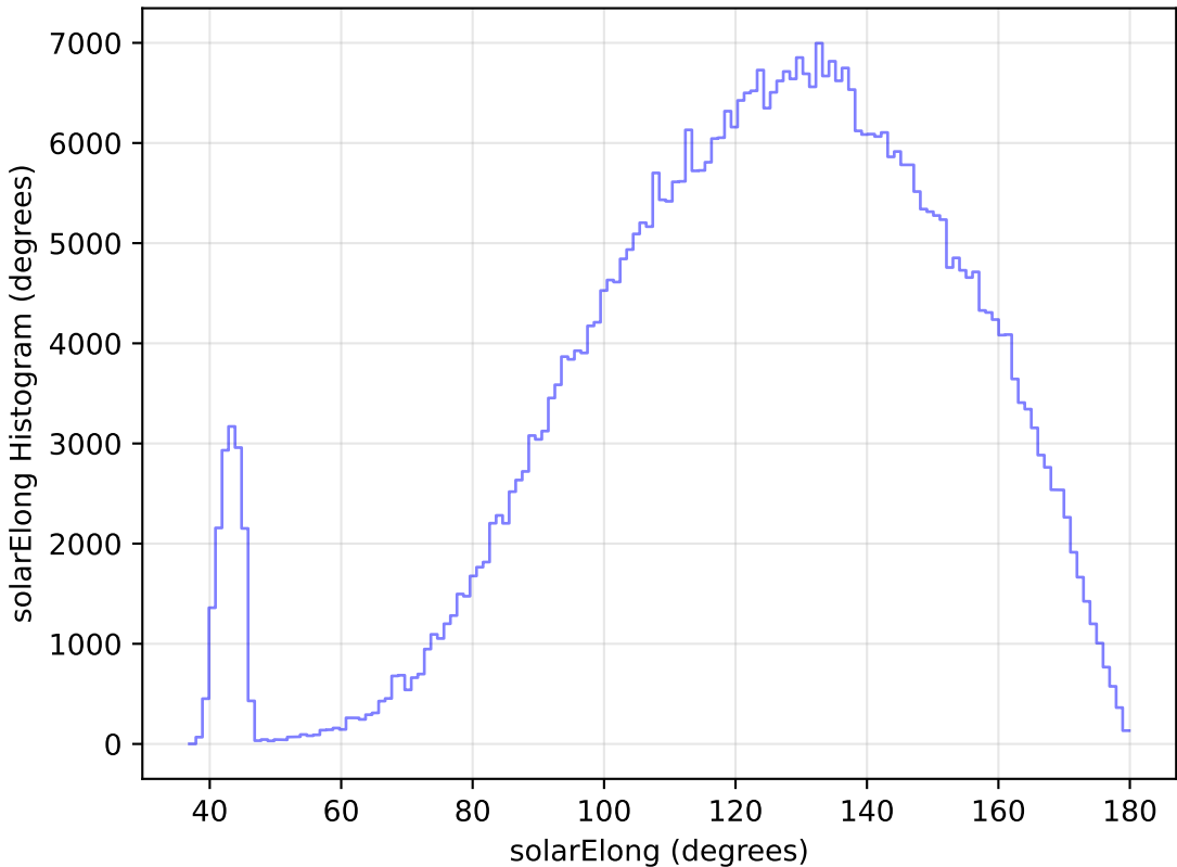
roll_pause_mjdp120_v3.4_10yrs All sky r band: solarElong Histogram
