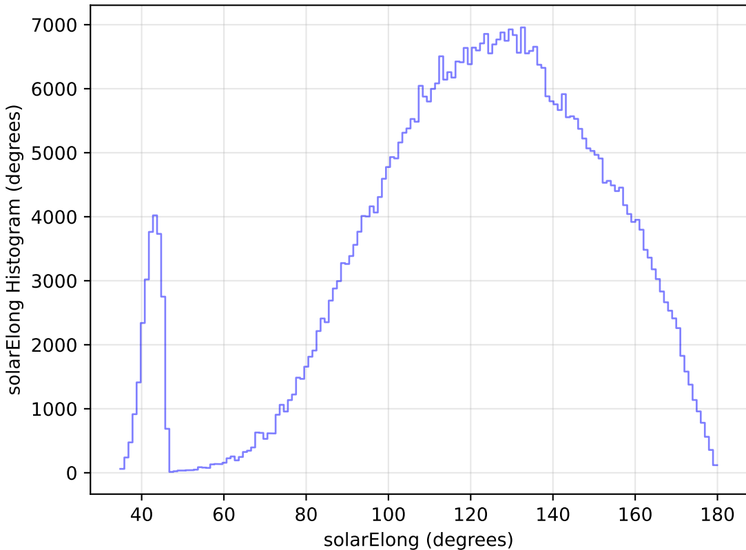
roll_pause_mjdp120_v3.4_10yrs All sky i band: solarElong Histogram
