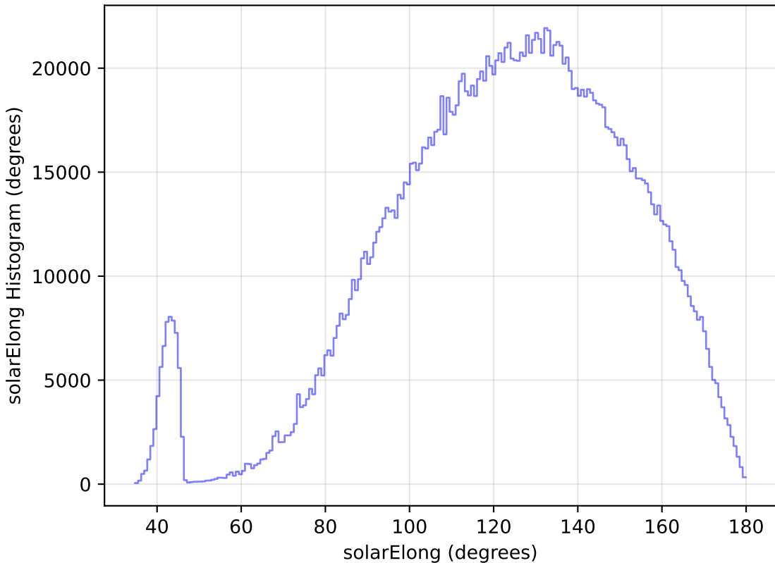
roll_pause_mjdp120_v3.4_10yrs All sky all bands: solarElong Histogram
