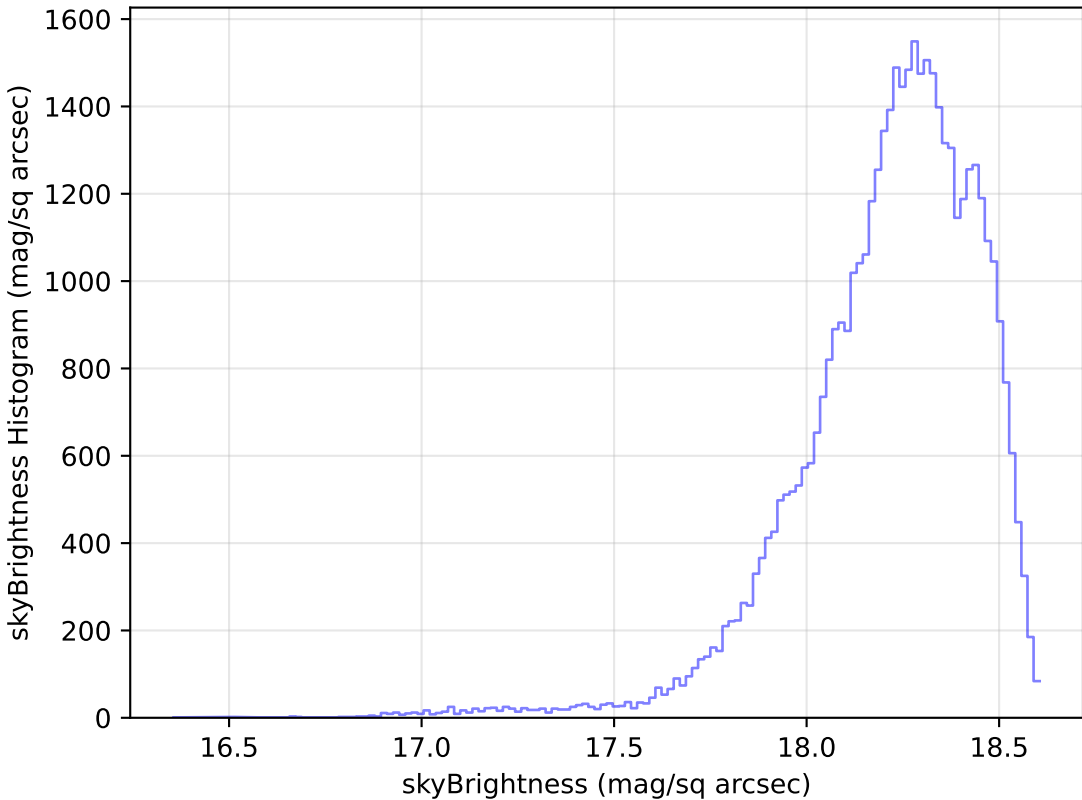
roll_pause_mjdp120_v3.4_10yrs Yr 1 y band: skyBrightness Histogram
