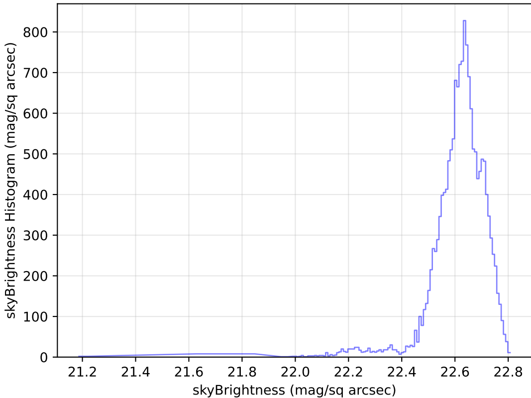
roll_pause_mjdp120_v3.4_10yrs Yr 1 u band: skyBrightness Histogram
