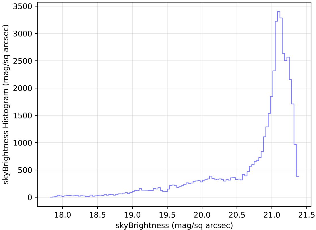
roll_pause_mjdp120_v3.4_10yrs Yr 1 r band: skyBrightness Histogram
