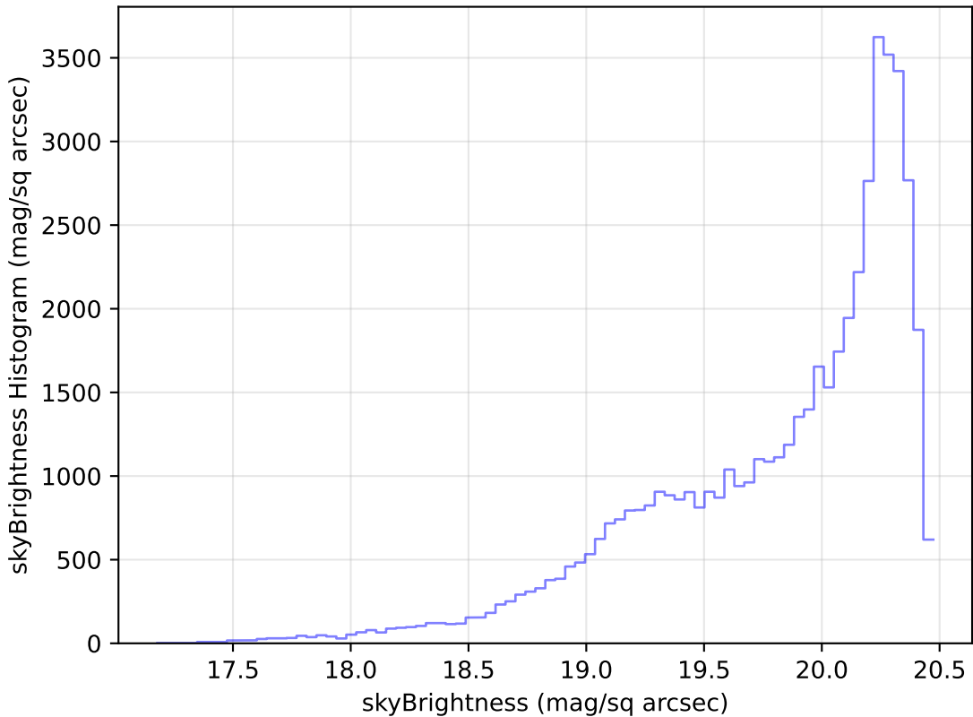
roll_pause_mjdp120_v3.4_10yrs Yr 1 i band: skyBrightness Histogram
