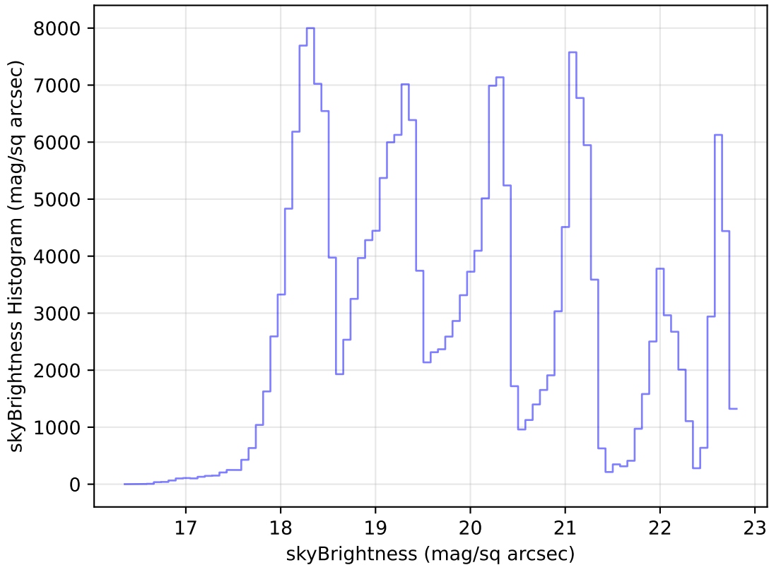
roll_pause_mjdp120_v3.4_10yrs Yr 1 all bands: skyBrightness Histogram
