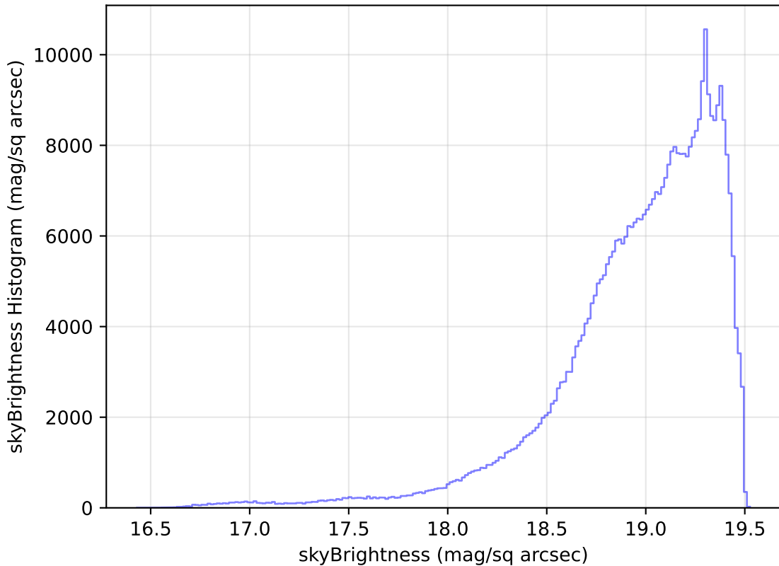
roll_pause_mjdp120_v3.4_10yrs WFD z band: skyBrightness Histogram
