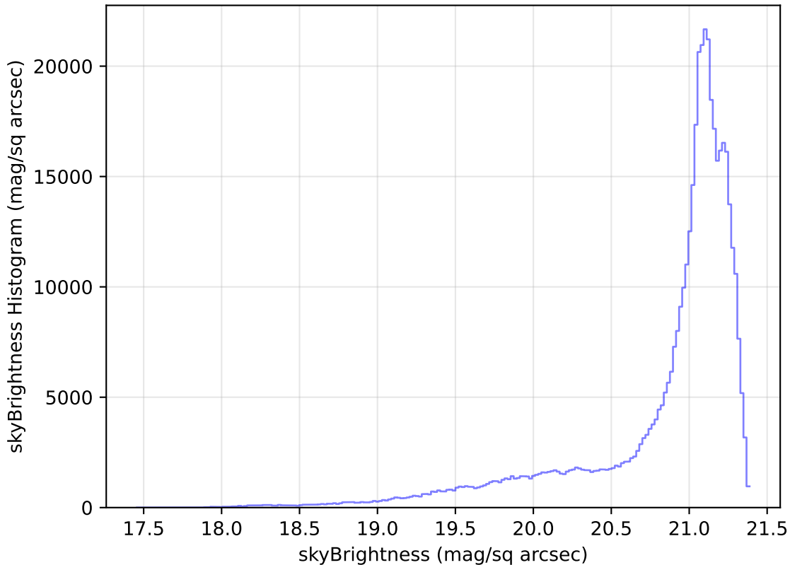
roll_pause_mjdp120_v3.4_10yrs WFD r band: skyBrightness Histogram
