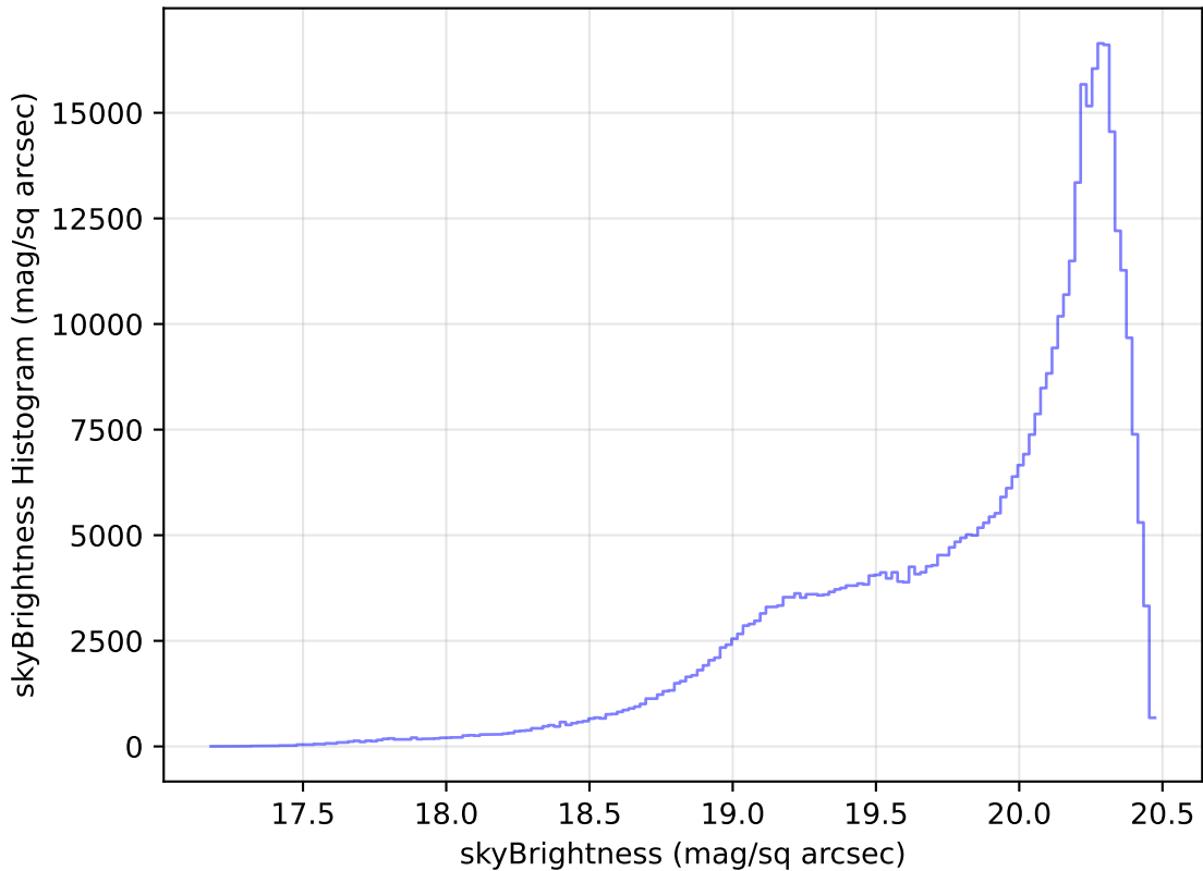
roll_pause_mjdp120_v3.4_10yrs WFD i band: skyBrightness Histogram
