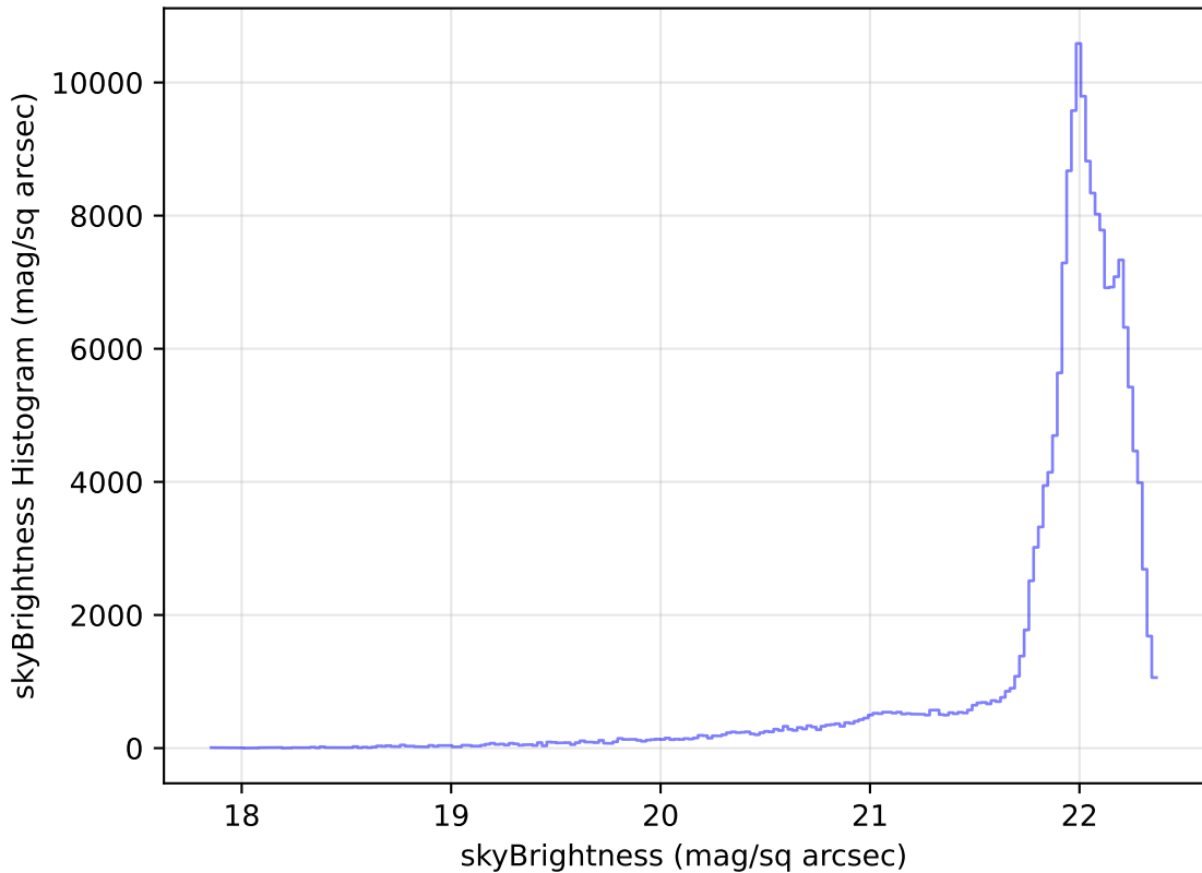
roll_pause_mjdp120_v3.4_10yrs WFD g band: skyBrightness Histogram
