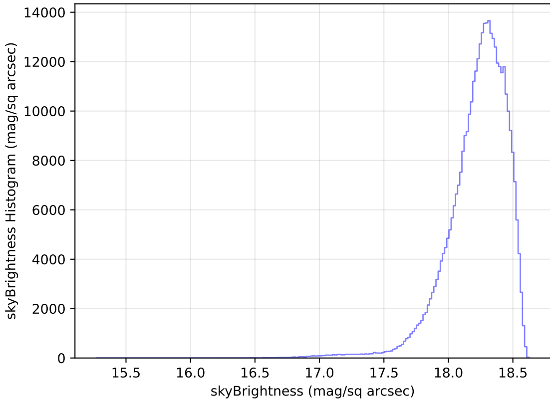
roll_pause_mjdp120_v3.4_10yrs All sky y band: skyBrightness Histogram
