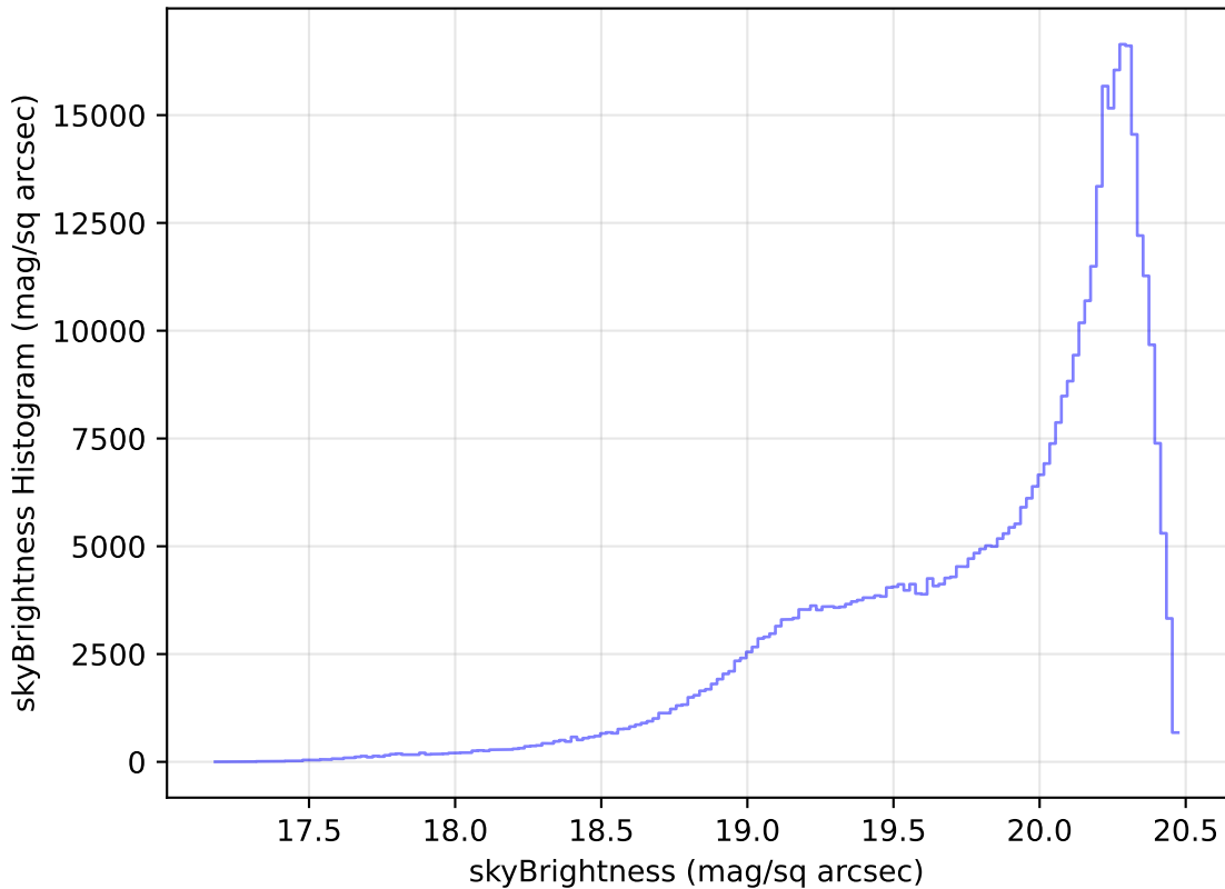
roll_pause_mjdp120_v3.4_10yrs All sky i band: skyBrightness Histogram
