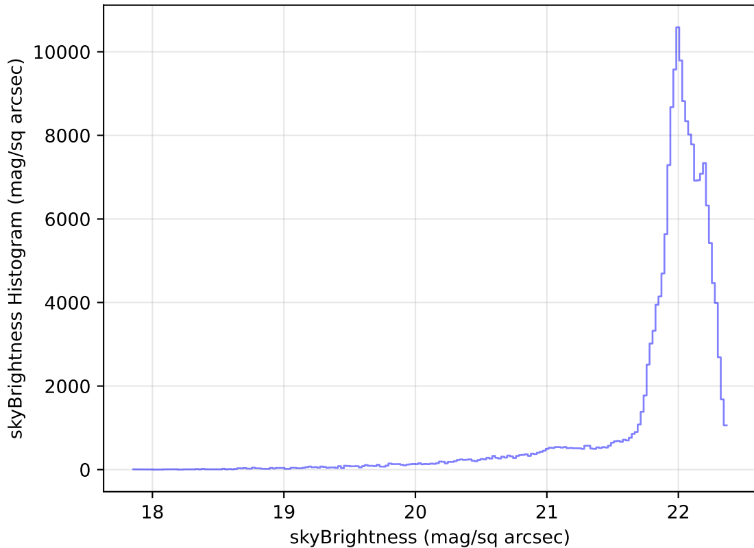
roll_pause_mjdp120_v3.4_10yrs All sky g band: skyBrightness Histogram
