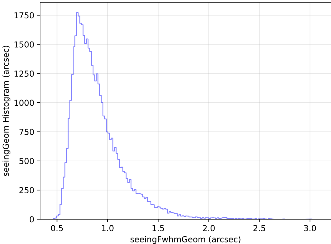
roll_pause_mjdp120_v3.4_10yrs Yr 1 z band: seeingGeom Histogram
