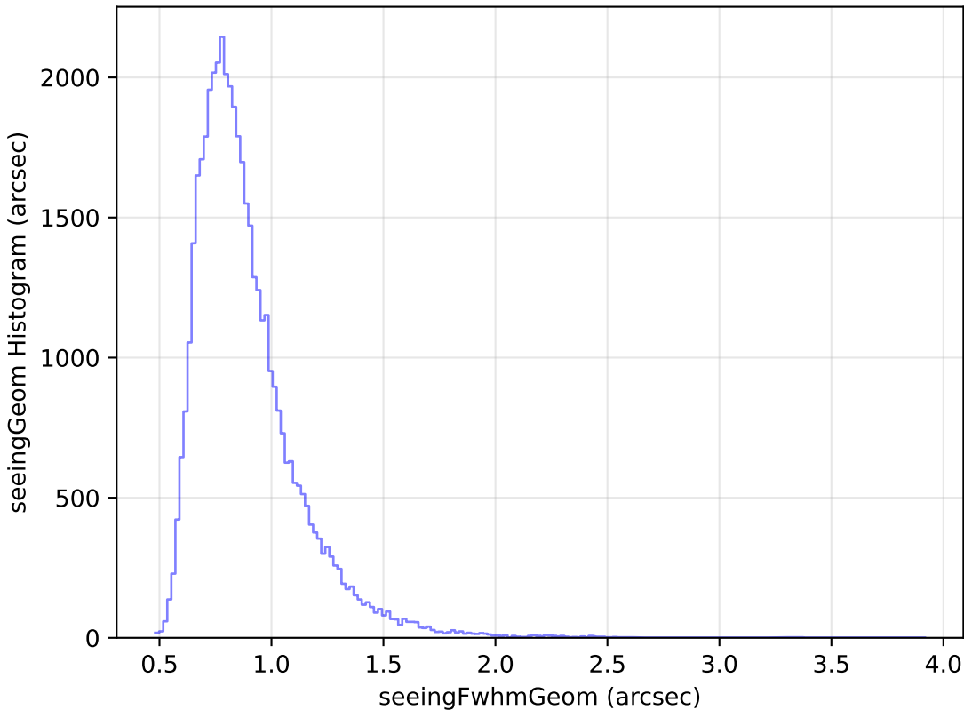
roll_pause_mjdp120_v3.4_10yrs Yr 1 y band: seeingGeom Histogram
