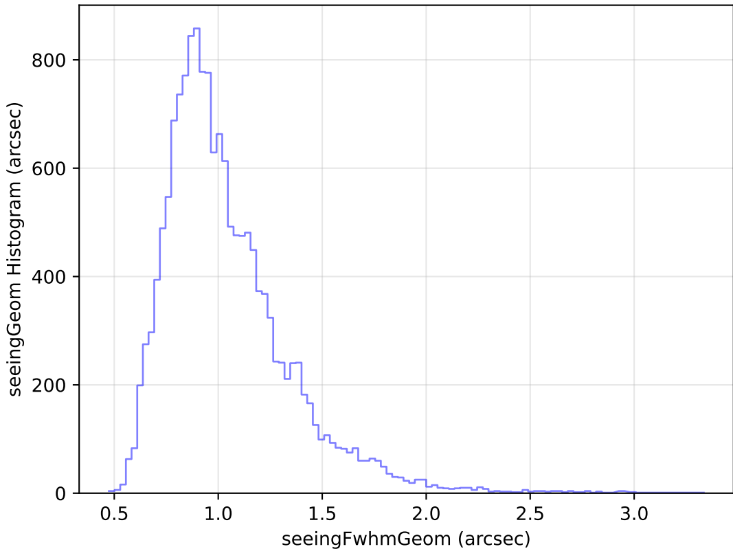
roll_pause_mjdp120_v3.4_10yrs Yr 1 u band: seeingGeom Histogram
