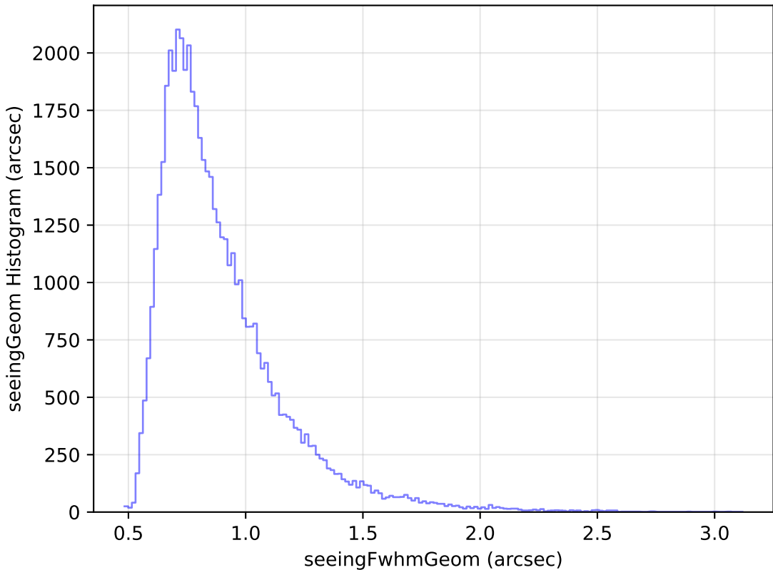
roll_pause_mjdp120_v3.4_10yrs Yr 1 i band: seeingGeom Histogram
