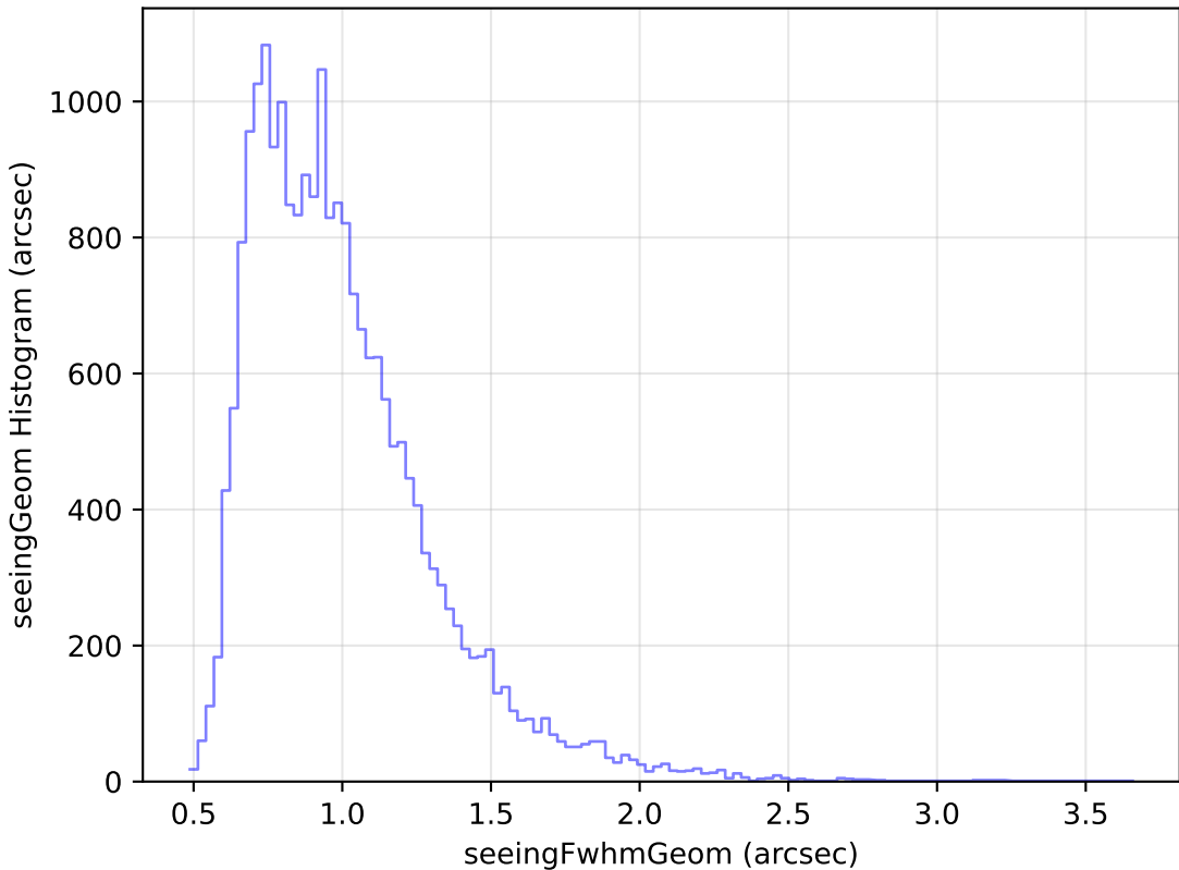
roll_pause_mjdp120_v3.4_10yrs Yr 1 g band: seeingGeom Histogram
