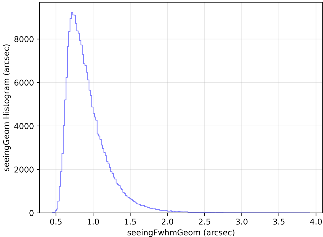
roll_pause_mjdp120_v3.4_10yrs Yr 1 all bands: seeingGeom Histogram
