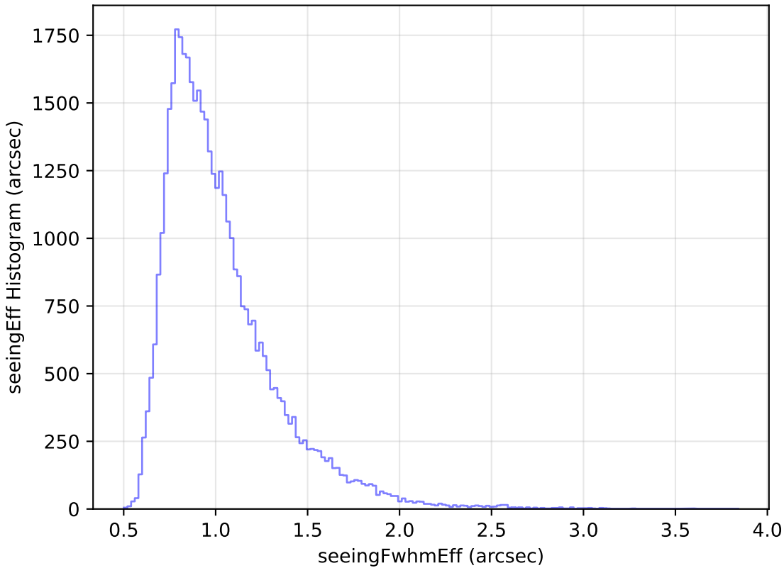
roll_pause_mjdp120_v3.4_10yrs Yr 1 z band: seeingEff Histogram
