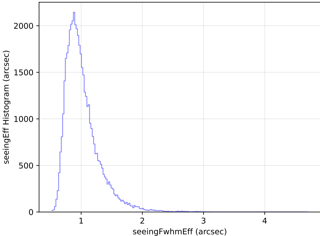
roll_pause_mjdp120_v3.4_10yrs Yr 1 y band: seeingEff Histogram
