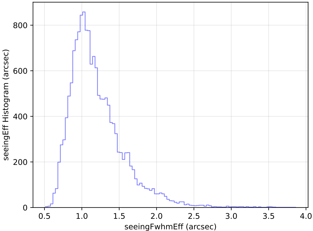
roll_pause_mjdp120_v3.4_10yrs Yr 1 u band: seeingEff Histogram
