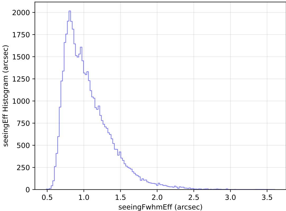
roll_pause_mjdp120_v3.4_10yrs Yr 1 r band: seeingEff Histogram
