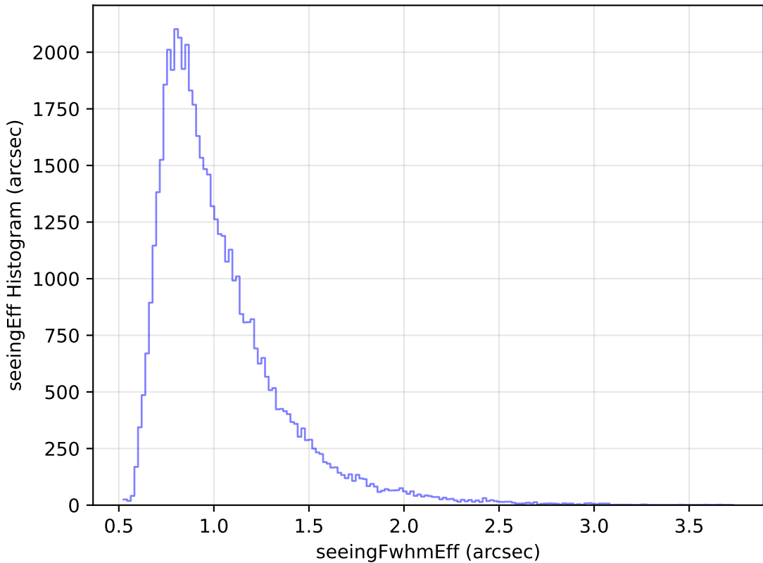
roll_pause_mjdp120_v3.4_10yrs Yr 1 i band: seeingEff Histogram
