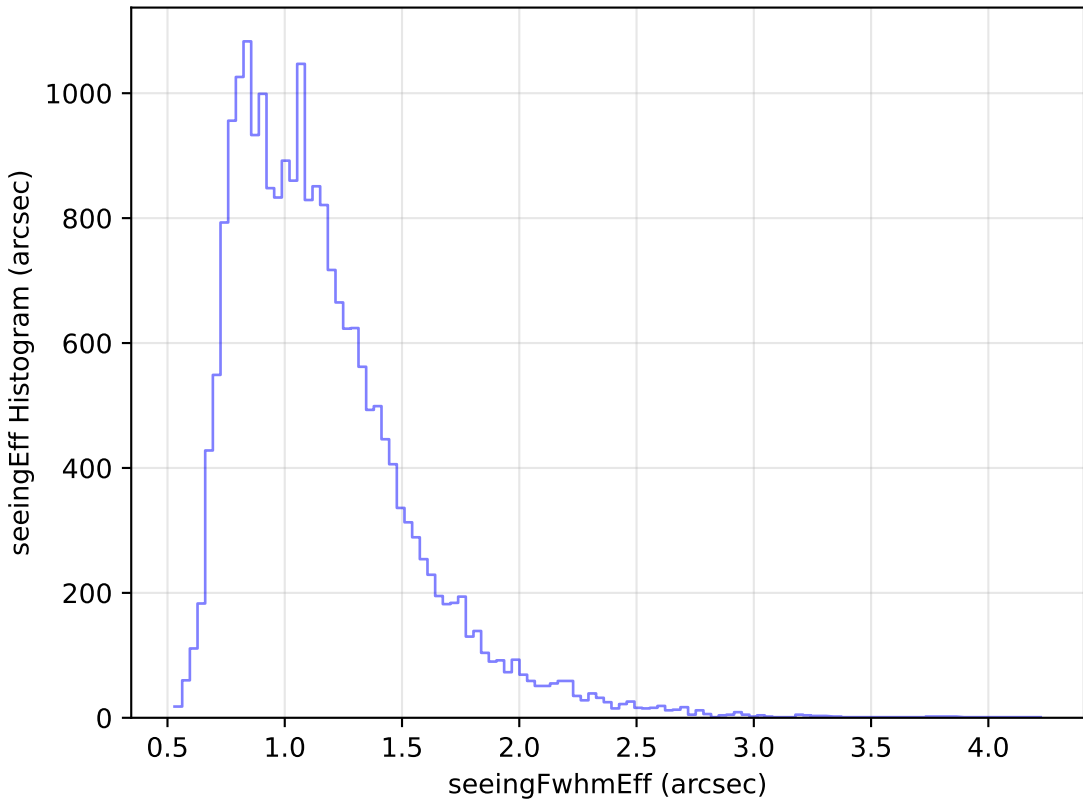
roll_pause_mjdp120_v3.4_10yrs Yr 1 g band: seeingEff Histogram
