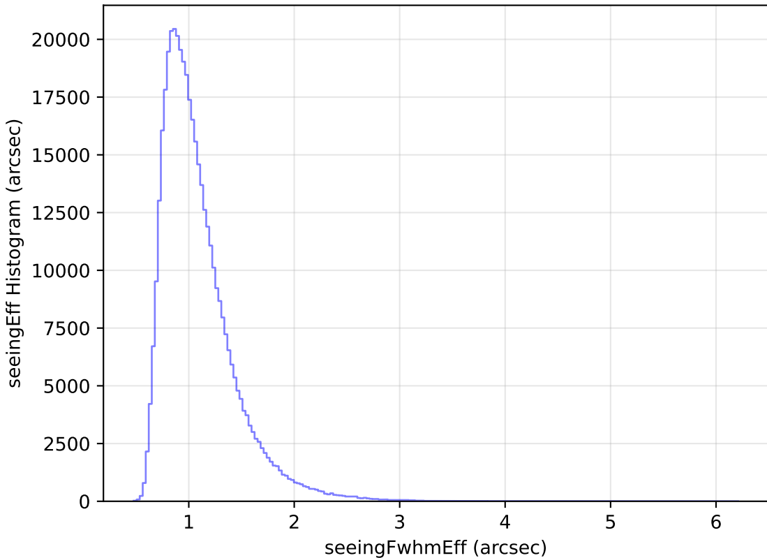
roll_pause_mjdp120_v3.4_10yrs WFD z band: seeingEff Histogram
