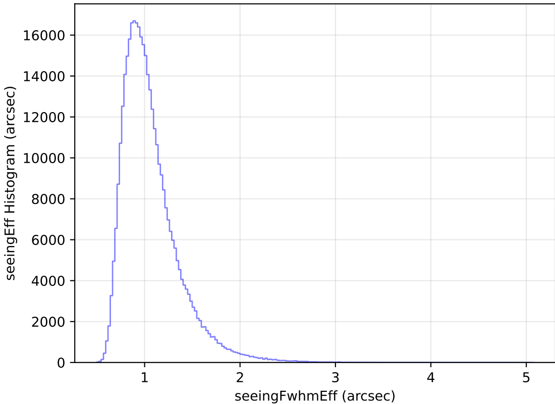
roll_pause_mjdp120_v3.4_10yrs WFD y band: seeingEff Histogram
